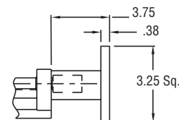
NEMA 34 Motor Adapter
